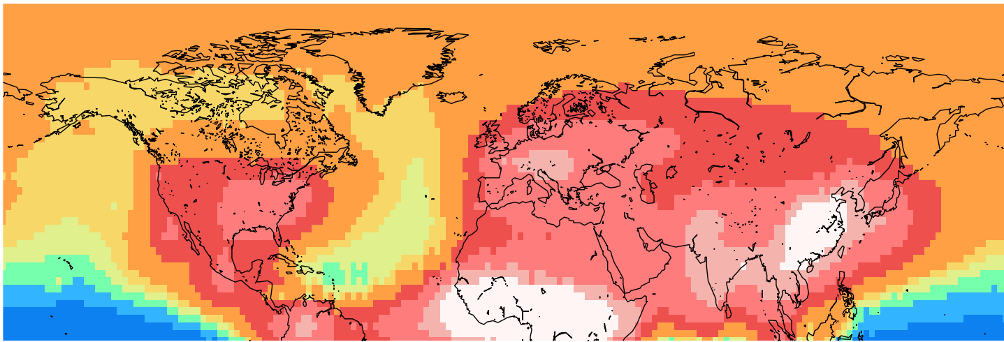
Black Carbon Optical Thickness ( \tau \times 100 )
