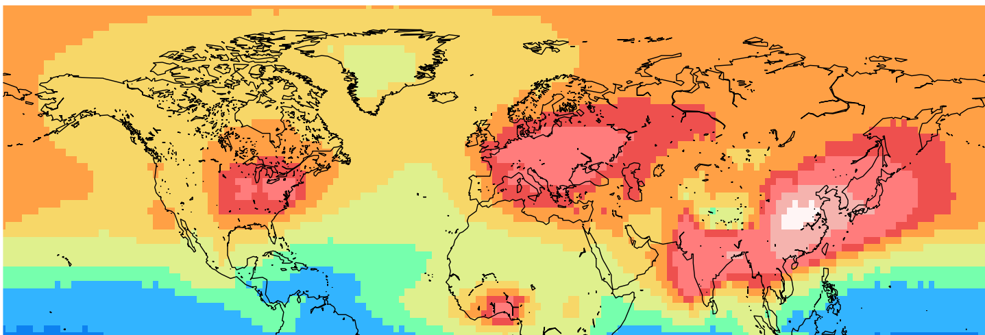
Surface Black Carbon Concentration ( \text{ng}/\text{m}^3 )
